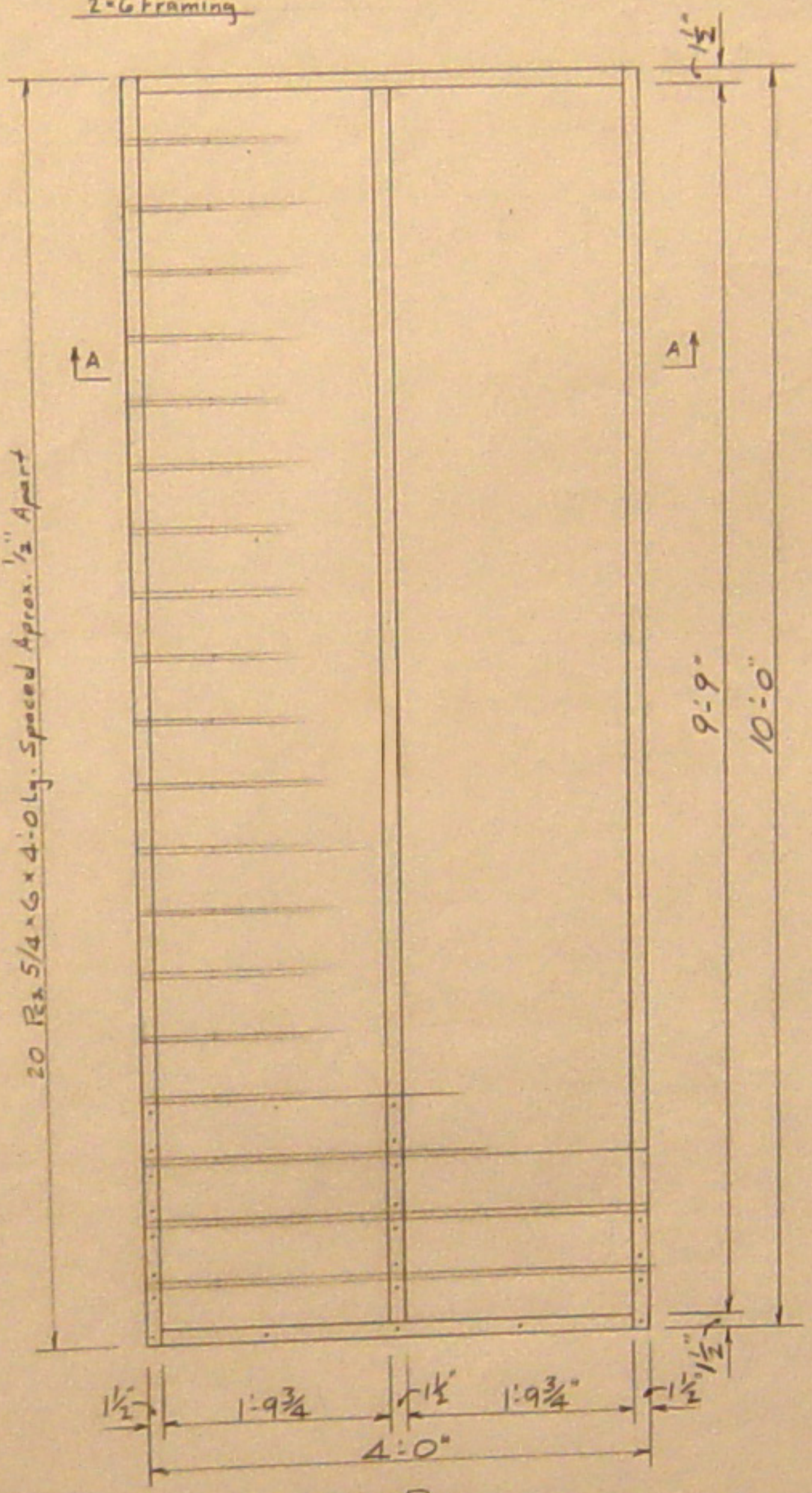
FRAMING PLAN
