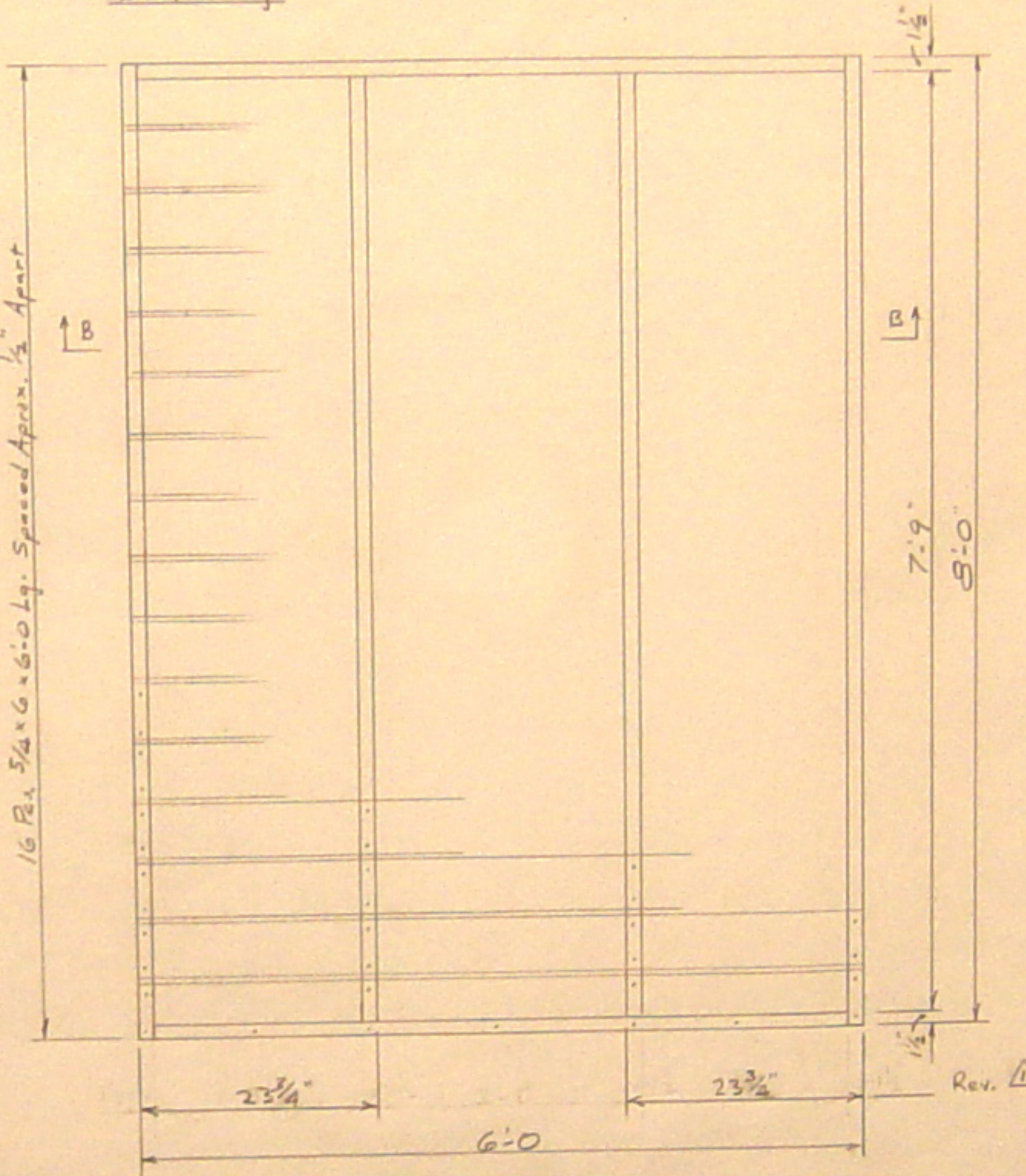
FRAMING PLAN
